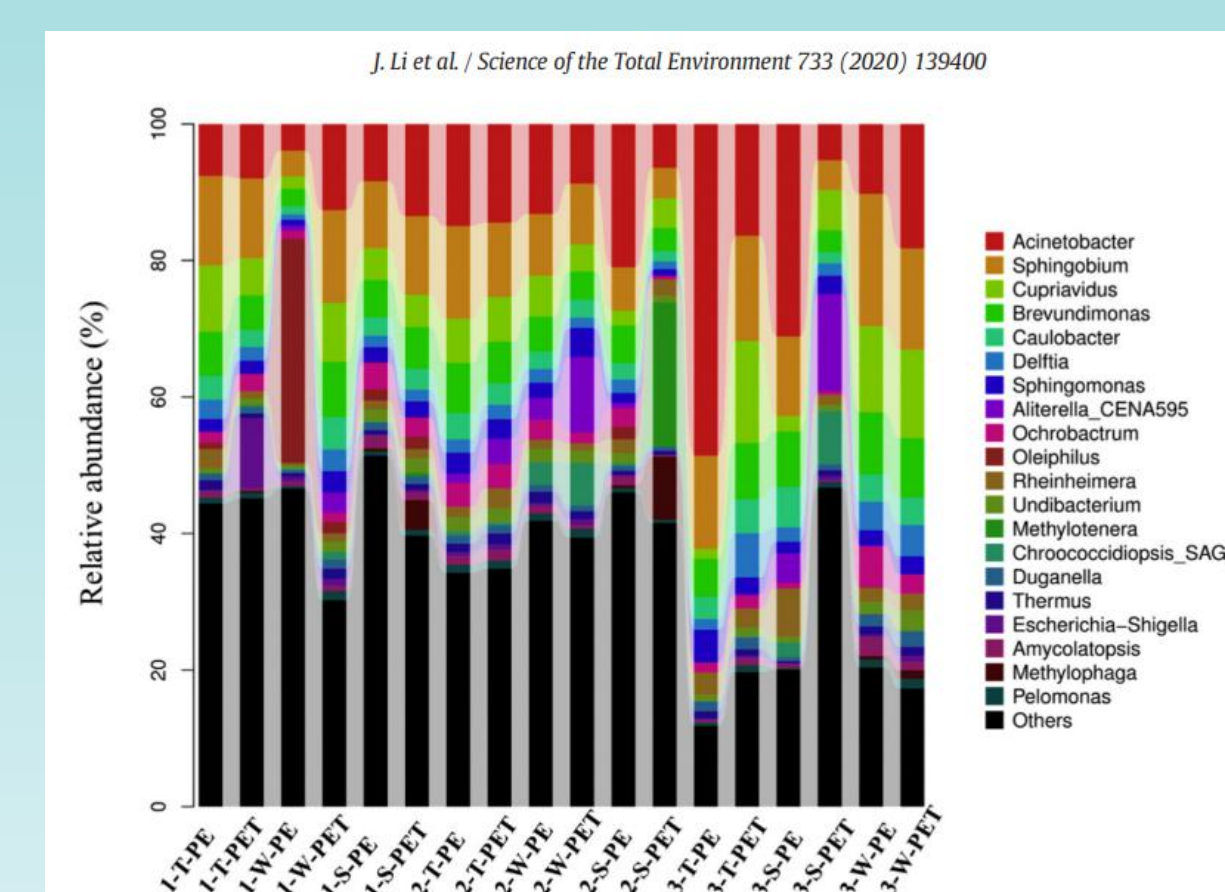
Fig. 4 Li, J., Huang, W., Jiang, R., Han, X., Zhang, D., & Zhang, C. (2020). The abundance of bacterial genera at three marine habitats over the sampling period. The Science of the Total Environment, 733, 139400. https://doi.org/10.1016/j.scitotenv.2020.139400
