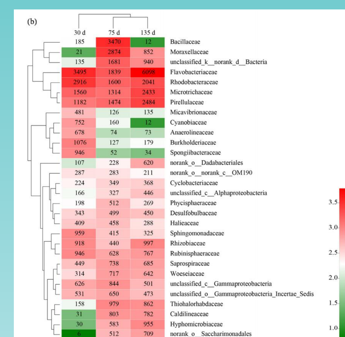
Fig. 3 Tu, C., Chen, T., Zhou, Q., Liu, Y., Wei, J., Wanik, J. J., & Luo, Y. (2020). Changes in the diversity of the microbial community structure for the PE associated biofilms. The Science of the Total Environment, 734, 139237. https://doi.org/10.1016/j.scitotenv.2020.139237
